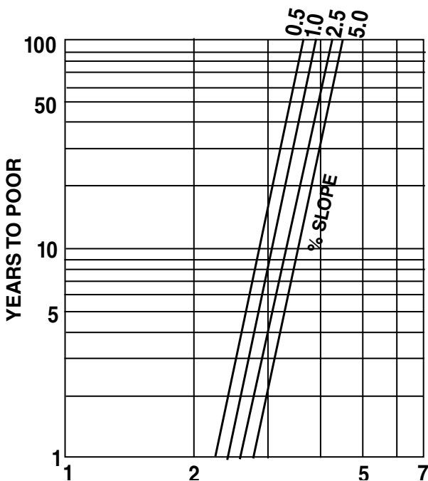
Figure 1: Concrete Pipe Culvert life
