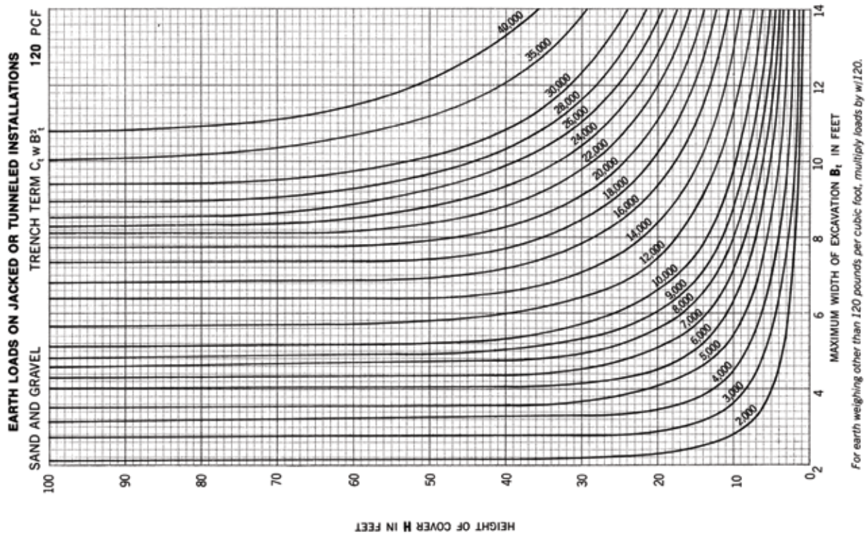
Figure 2 Earth Loads On Jacked or Tunneled Installations
