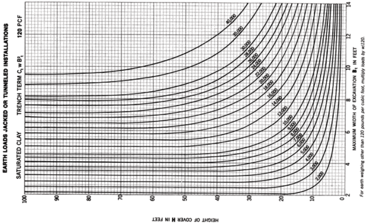
Figure 8 Earth Loads On Jacked or Tunneler Installations
